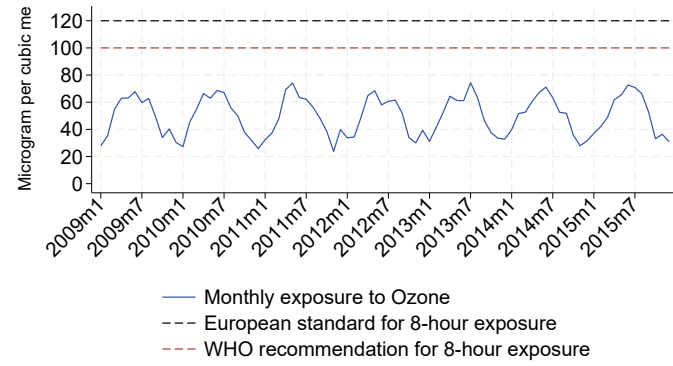
(b) Ozone
