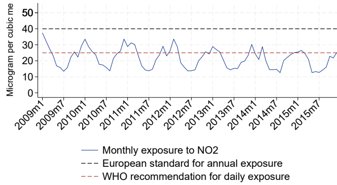
(a) NO 2
